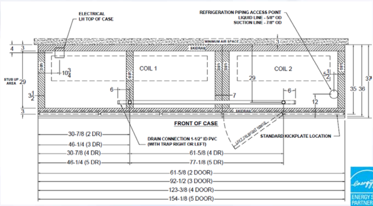
RN6SN Plan View
