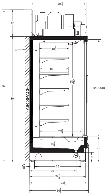
DN6LD CROSS VIEW
