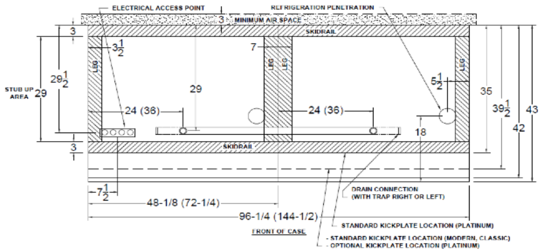
DX6HN PLAN VIEW
