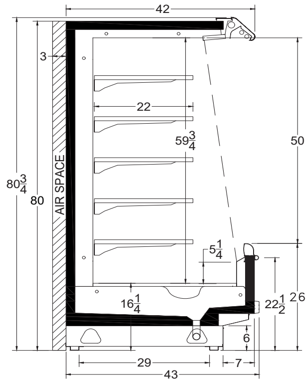
DX6HN CROSS VIEW
