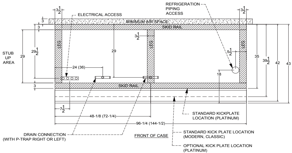
DX6LD PLAN VIEW
