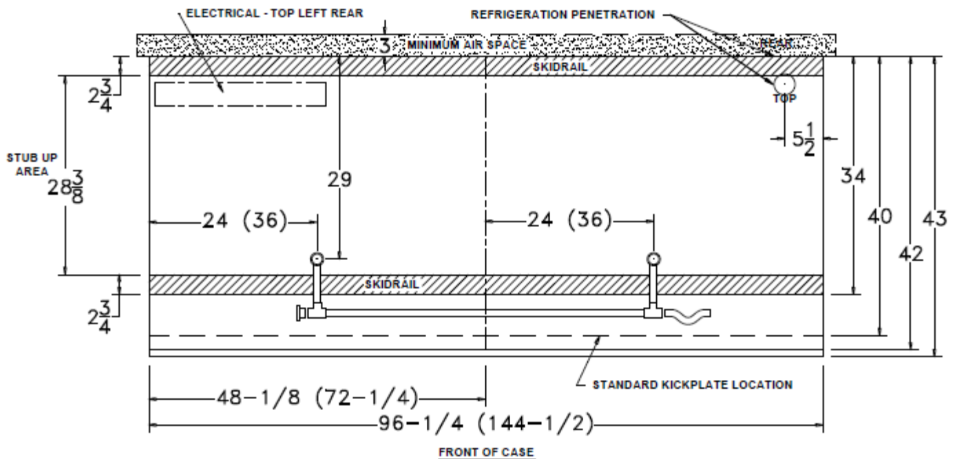
DX7 Ultra-Low Plan View
