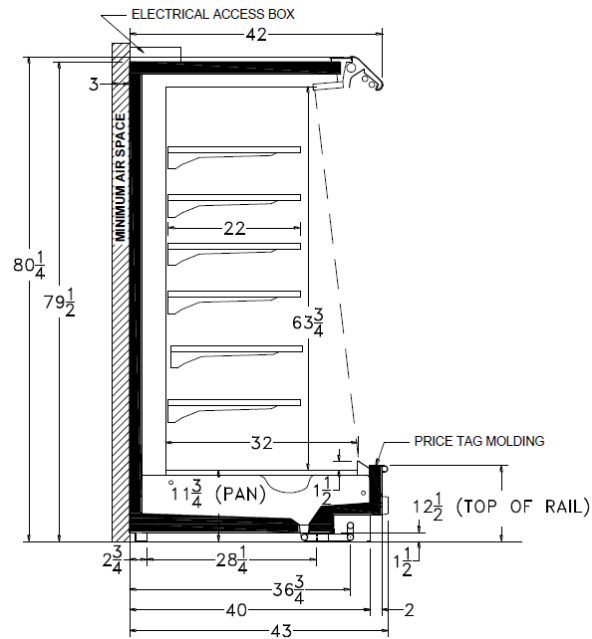
DX7UN Cross View
