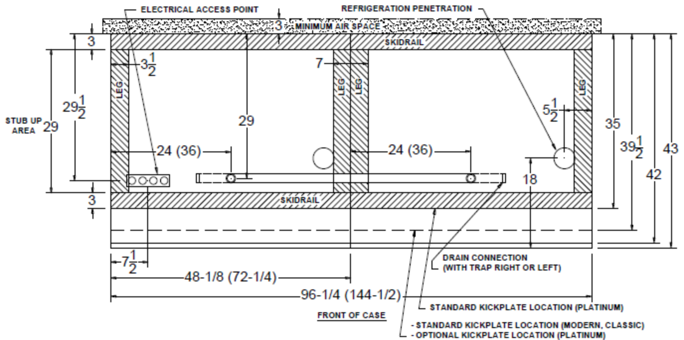
DX7 Ultra-Low Plan View
