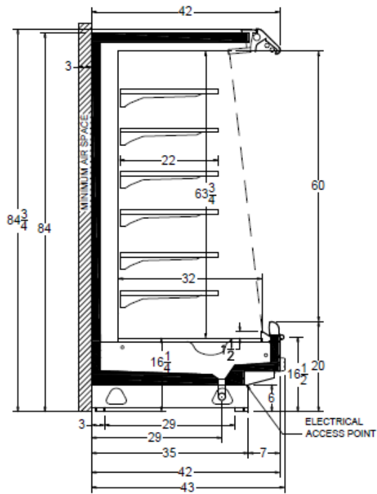
DX7LN Cross View
