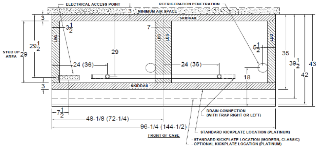
DX9LN PLAN VIEW
