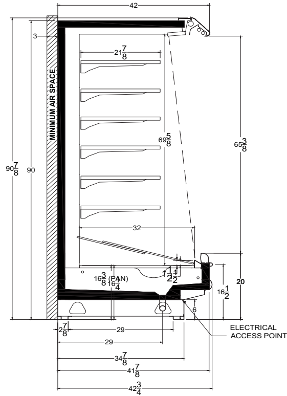
DX9LN CROSS VIEW
