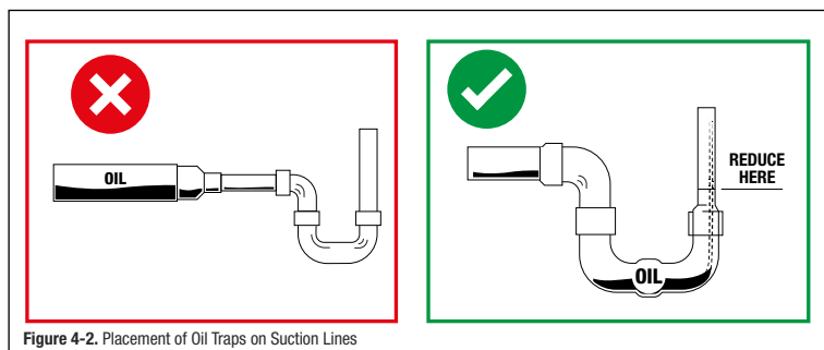
Figure 4-2. Placement of Oil Traps on Suction Lines
