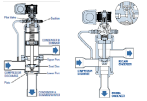
Figure 1-9. Heat reclaim 3-way valve split condenser valve
