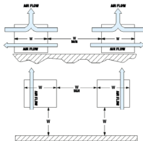
Figure 3-13. Minimum Clearance for Multiple Units
