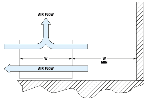
Figure 3-11. Minimum Distance from Walls and Obstructions
