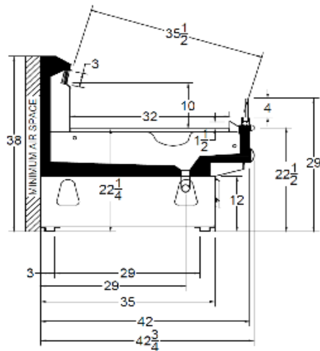
MX1LP CROSS VIEW
