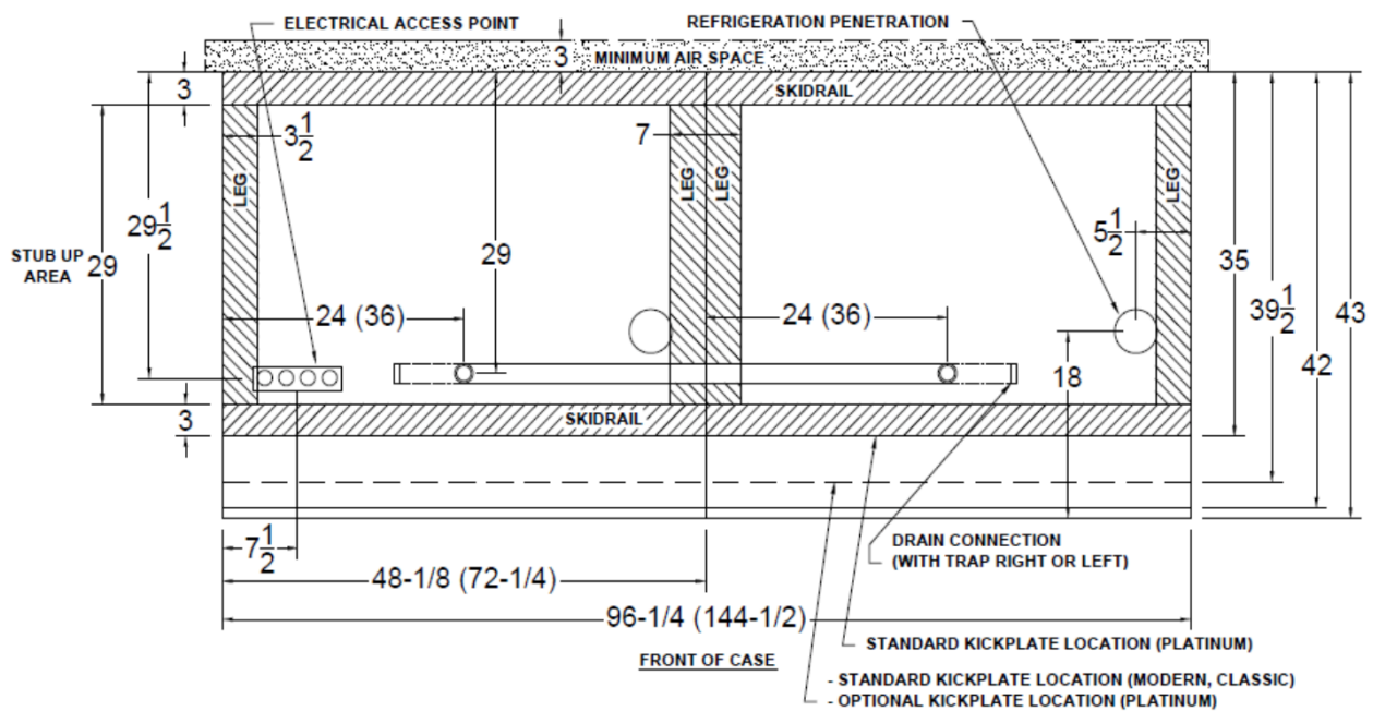
MX1LP PLAN VIEW
