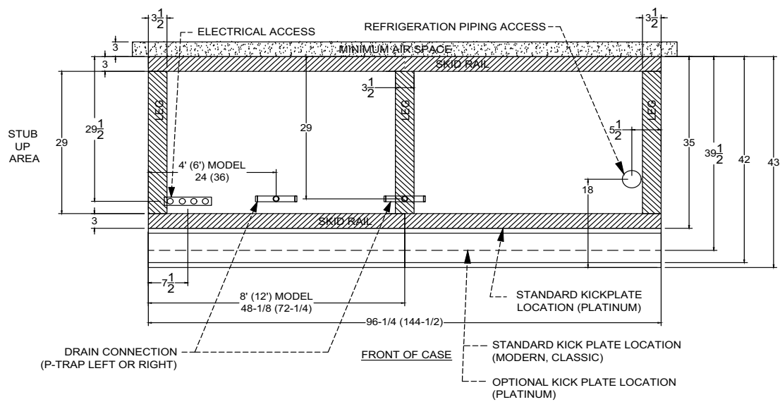
MX2LG PLAN VIEW (Single Coil)
