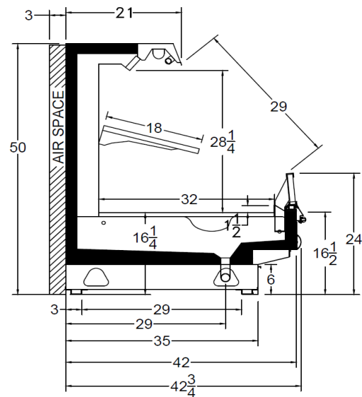
MX2LG CROSS VIEW
