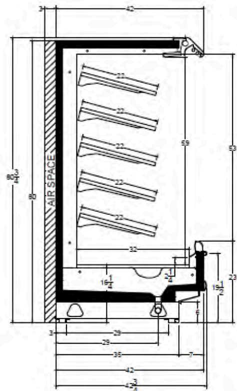
MX6XN Cross View
