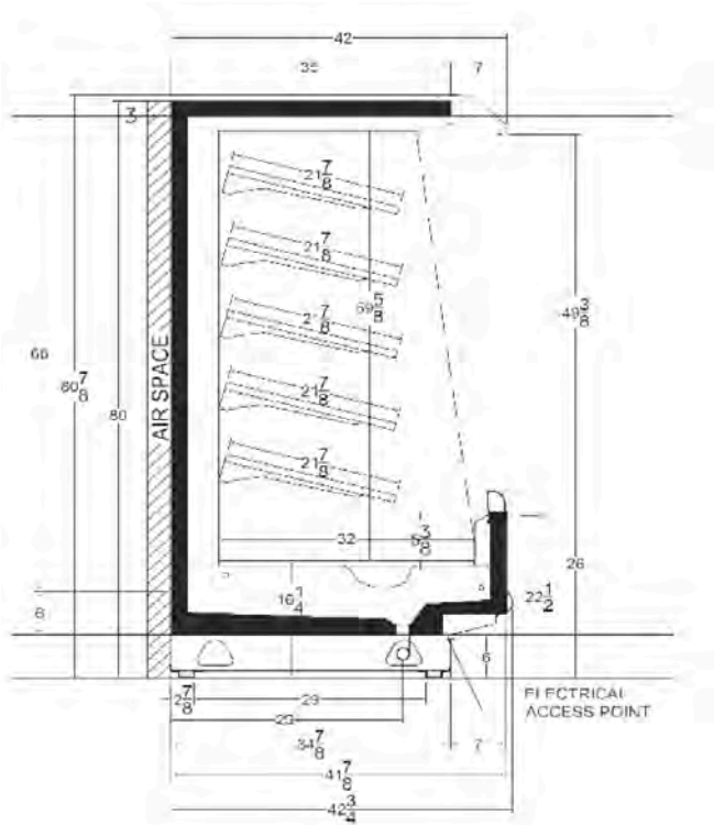
MX6HN Cross View
