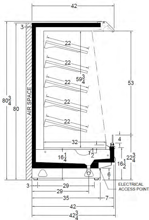
MX6LP Cross View
