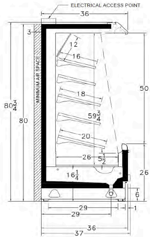
MN6HN Cross View
