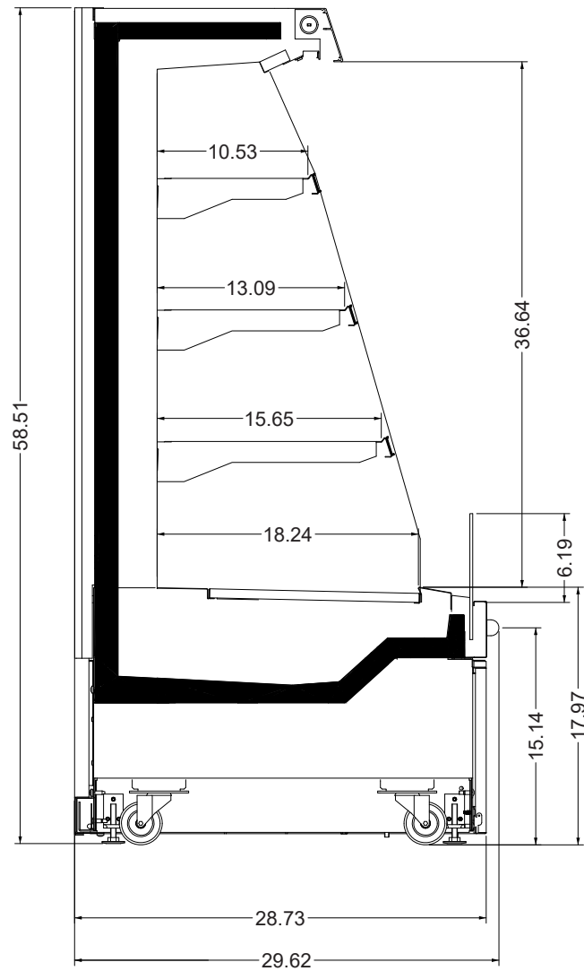
Section View
