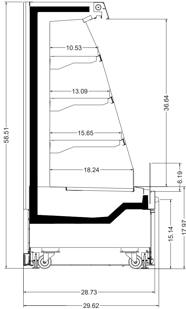
Section View
