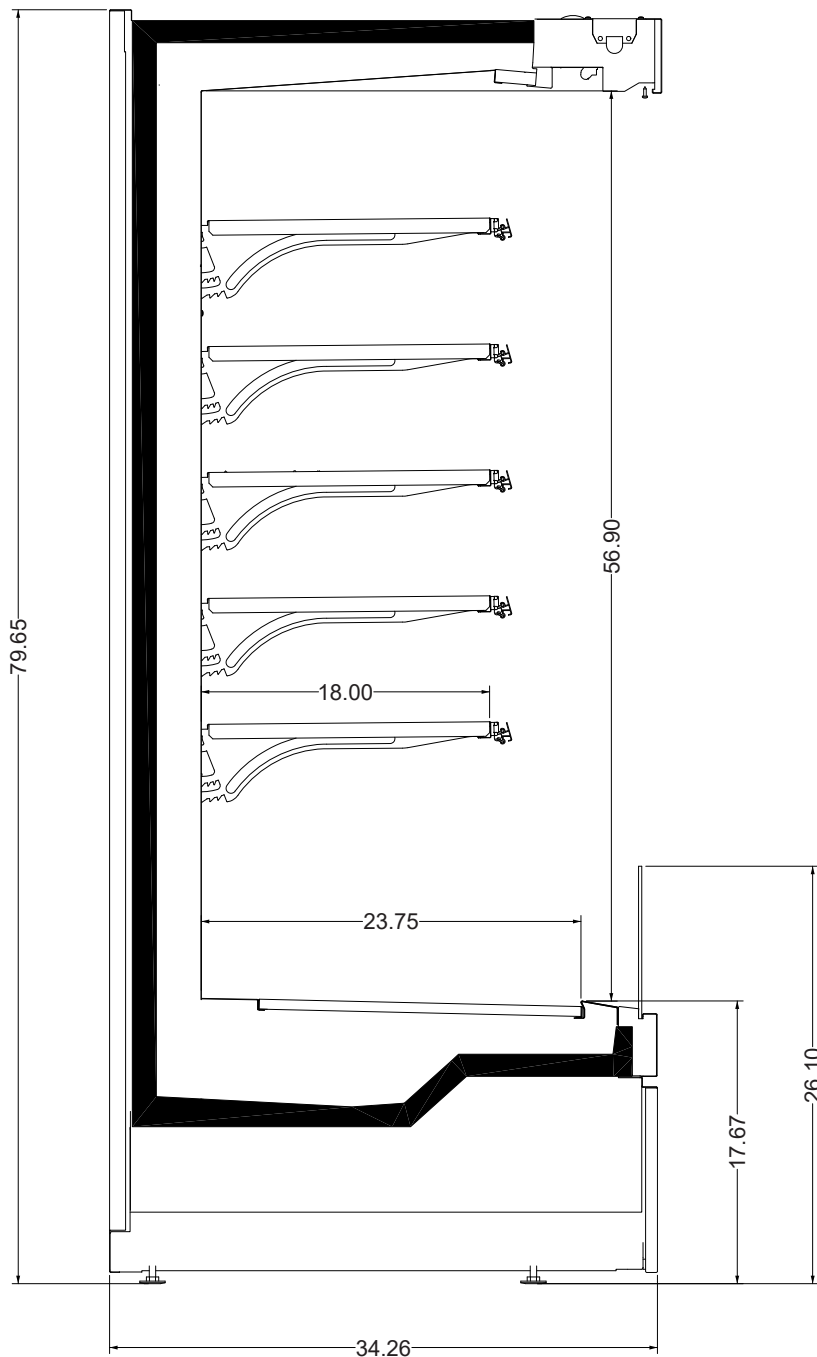
Section View
